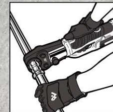
Press connection
